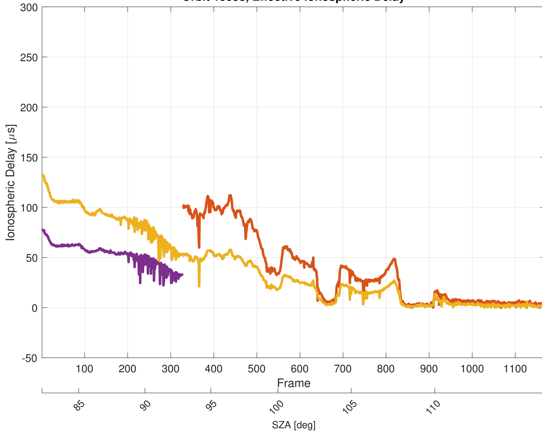
Orbit 15558, Effective Ionospheric Delay
