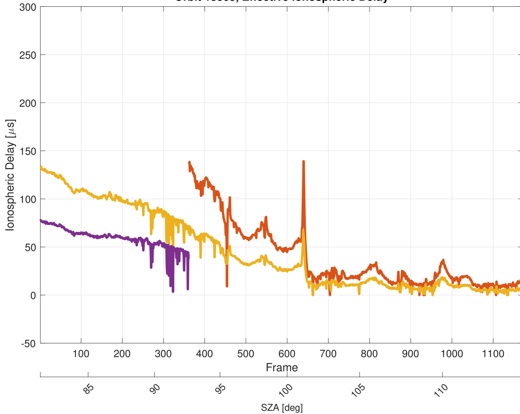
Orbit 15565, Effective Ionospheric Delay
