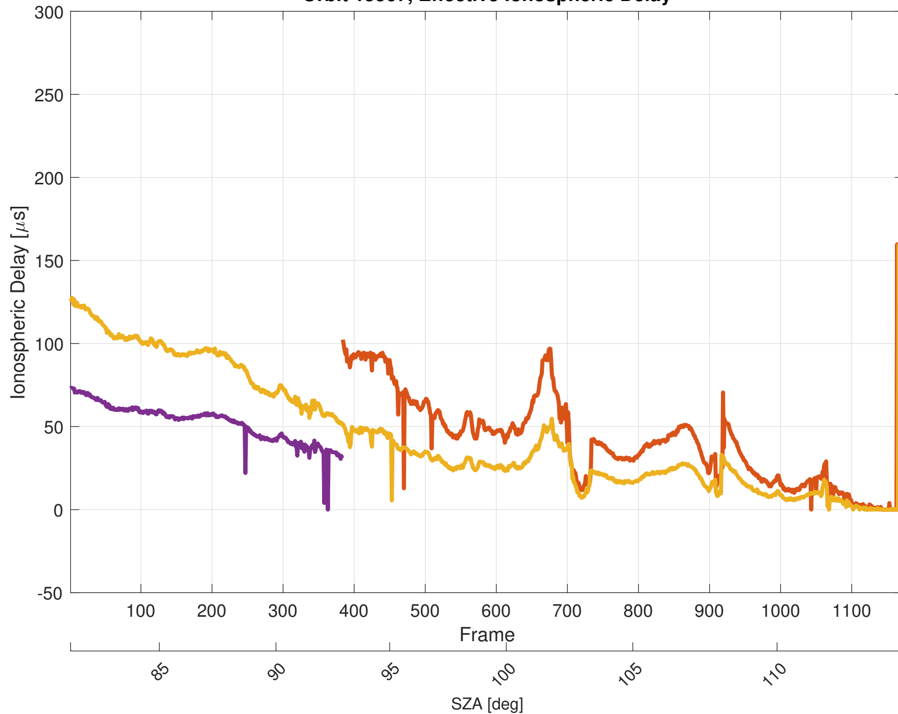
Orbit 15567, Effective Ionospheric Delay
