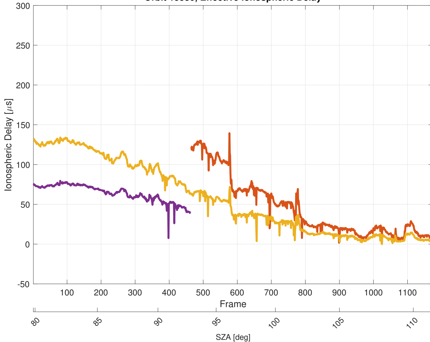
Orbit 15580, Effective Ionospheric Delay
