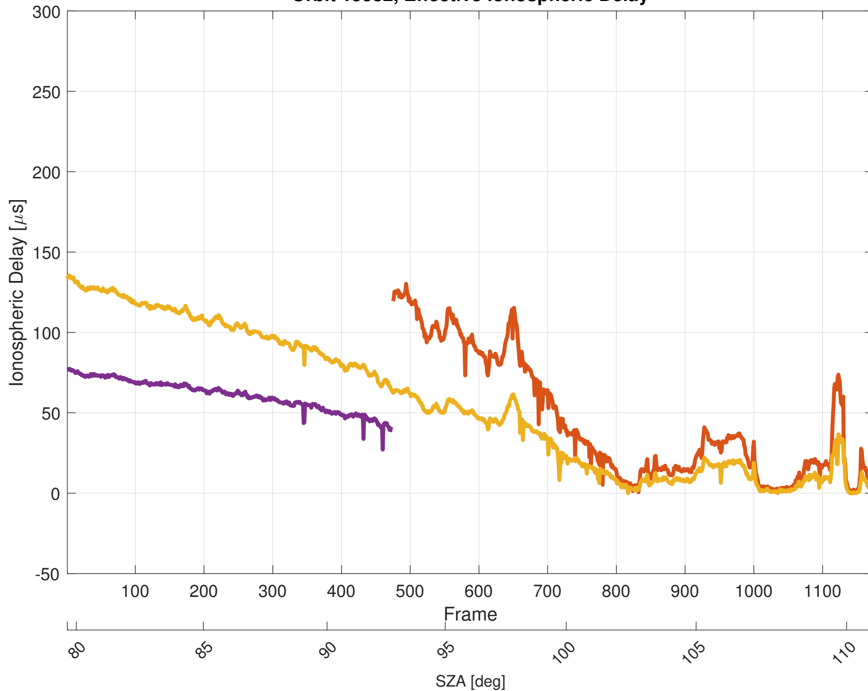
Orbit 15582, Effective Ionospheric Delay
