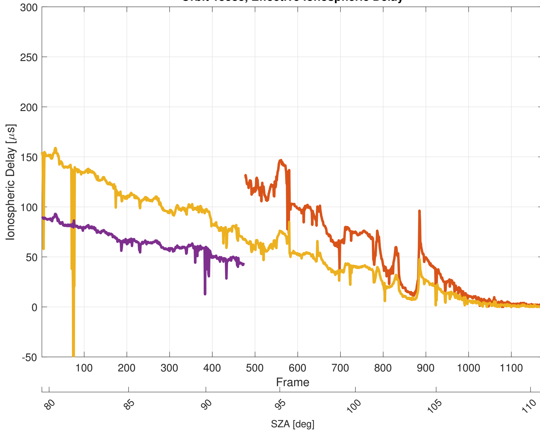
Orbit 15583, Effective Ionospheric Delay
