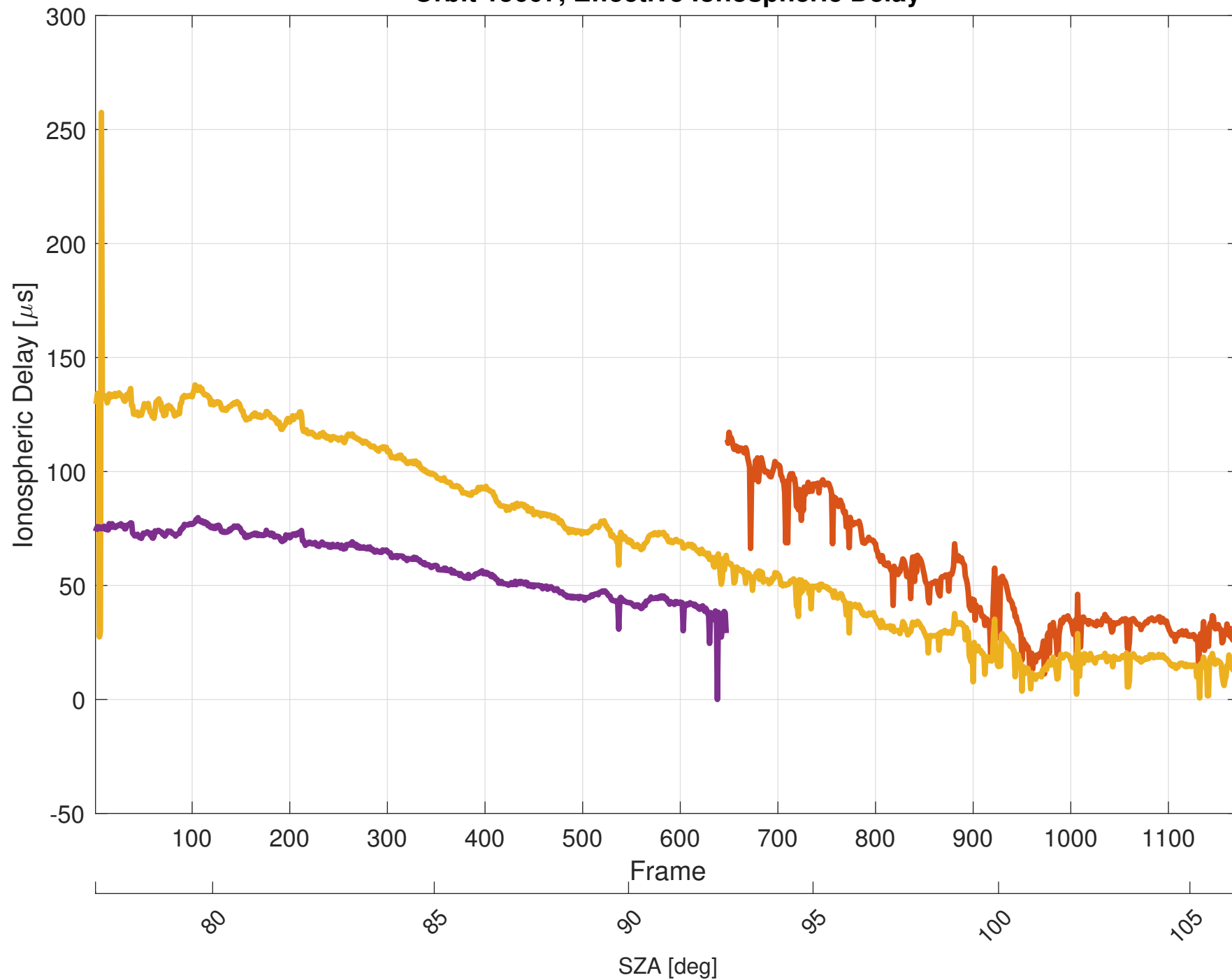
Orbit 15607, Effective Ionospheric Delay
