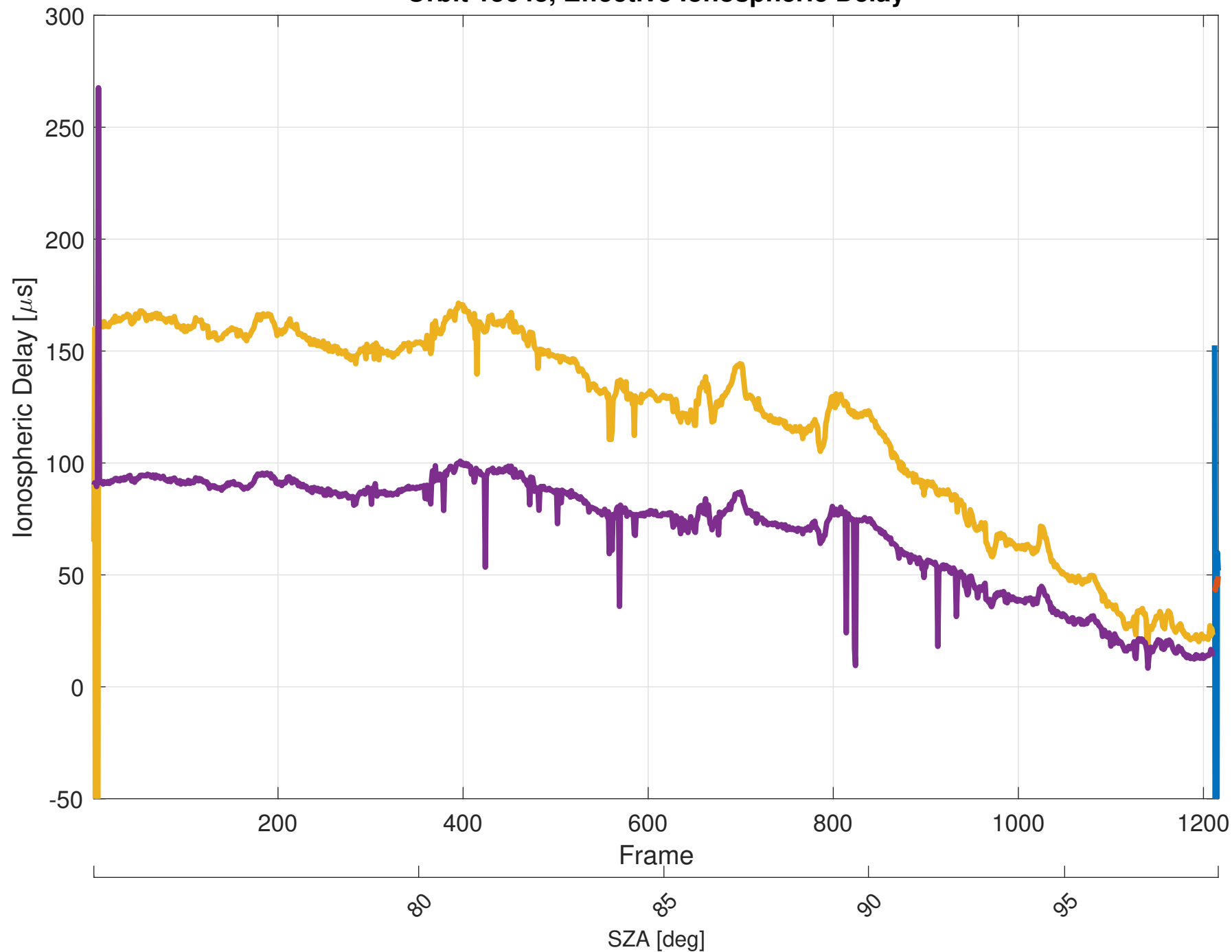
Orbit 15643, Effective Ionospheric Delay
