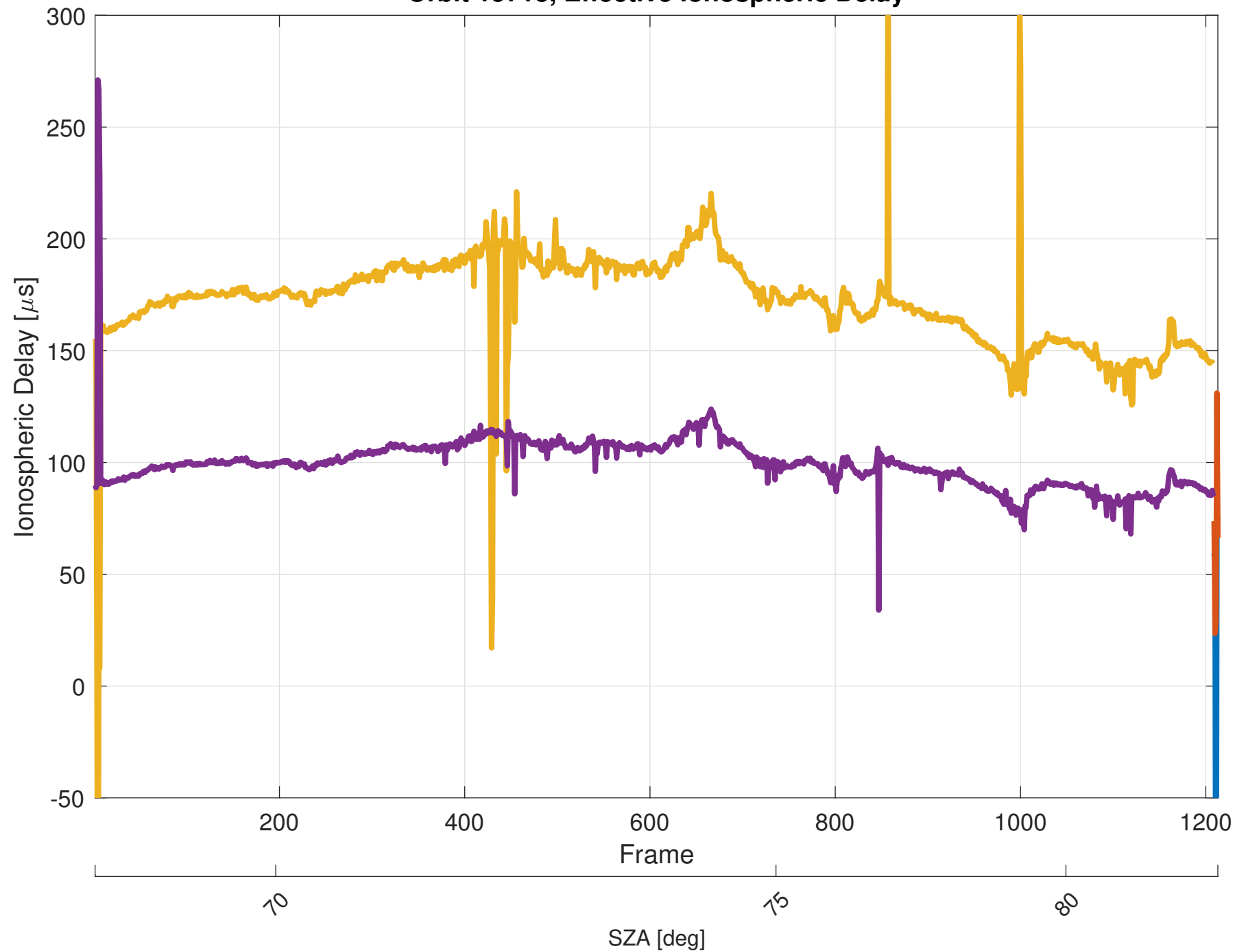
Orbit 15713, Effective Ionospheric Delay
