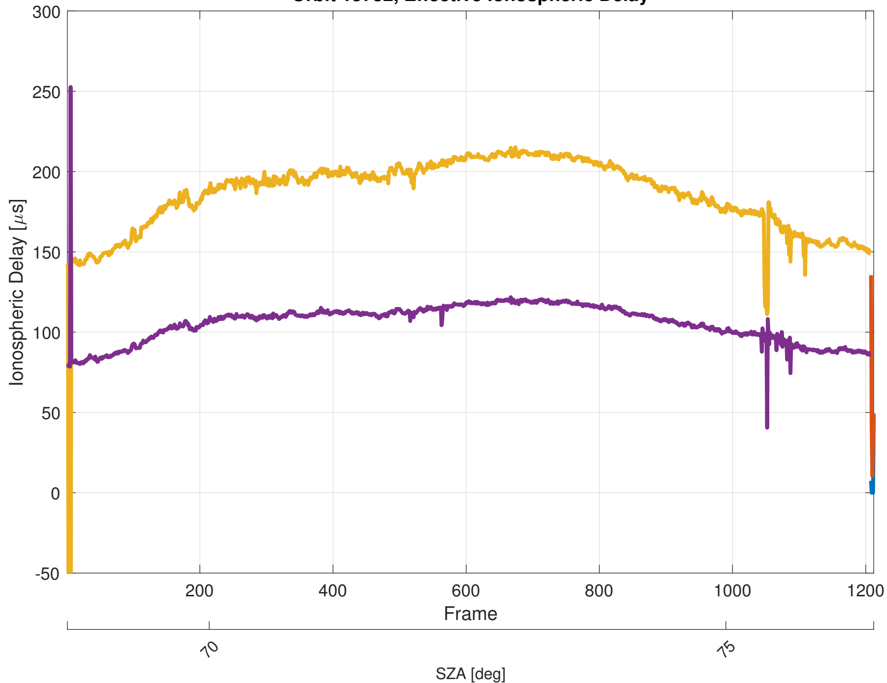
Orbit 15732, Effective Ionospheric Delay
