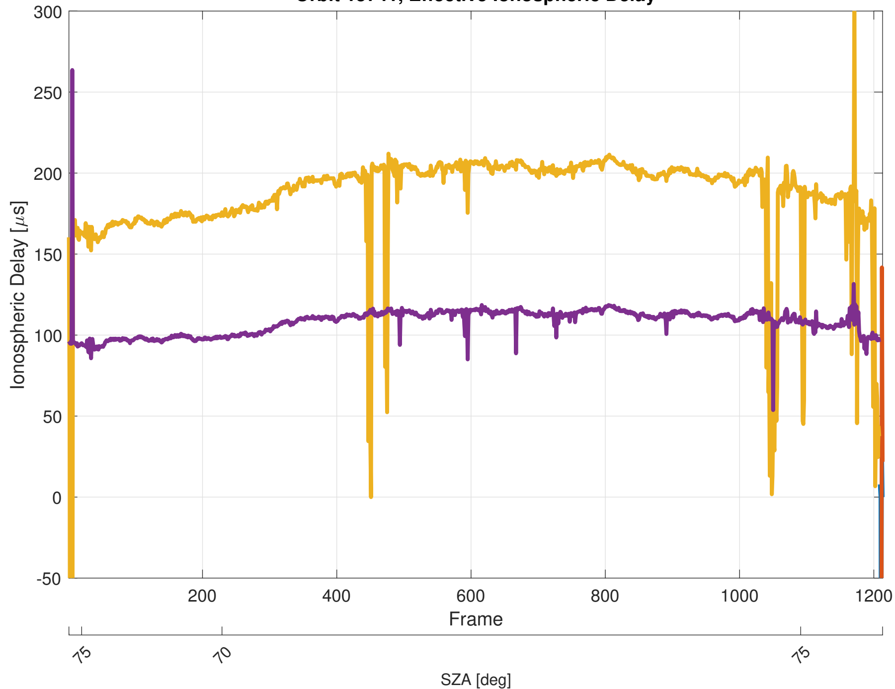
Orbit 15741, Effective Ionospheric Delay
