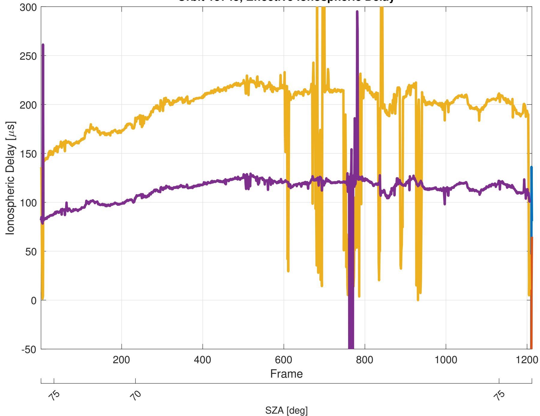
Orbit 15745, Effective Ionospheric Delay
