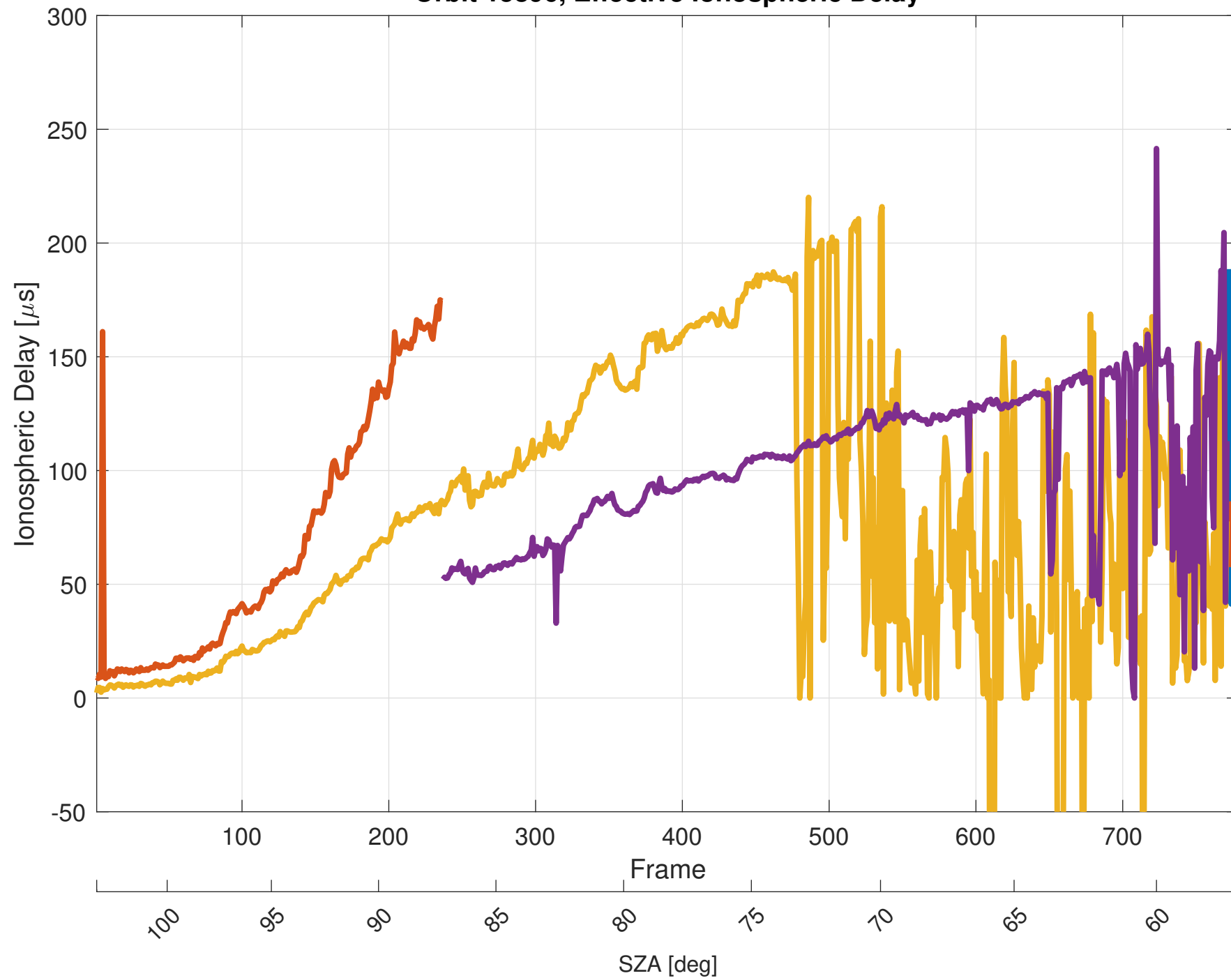
Orbit 15896, Effective Ionospheric Delay
