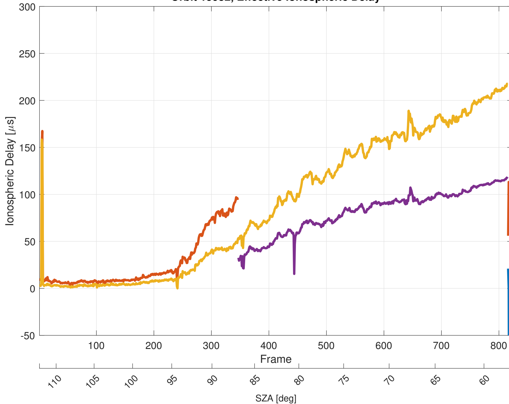
Orbit 15932, Effective Ionospheric Delay
