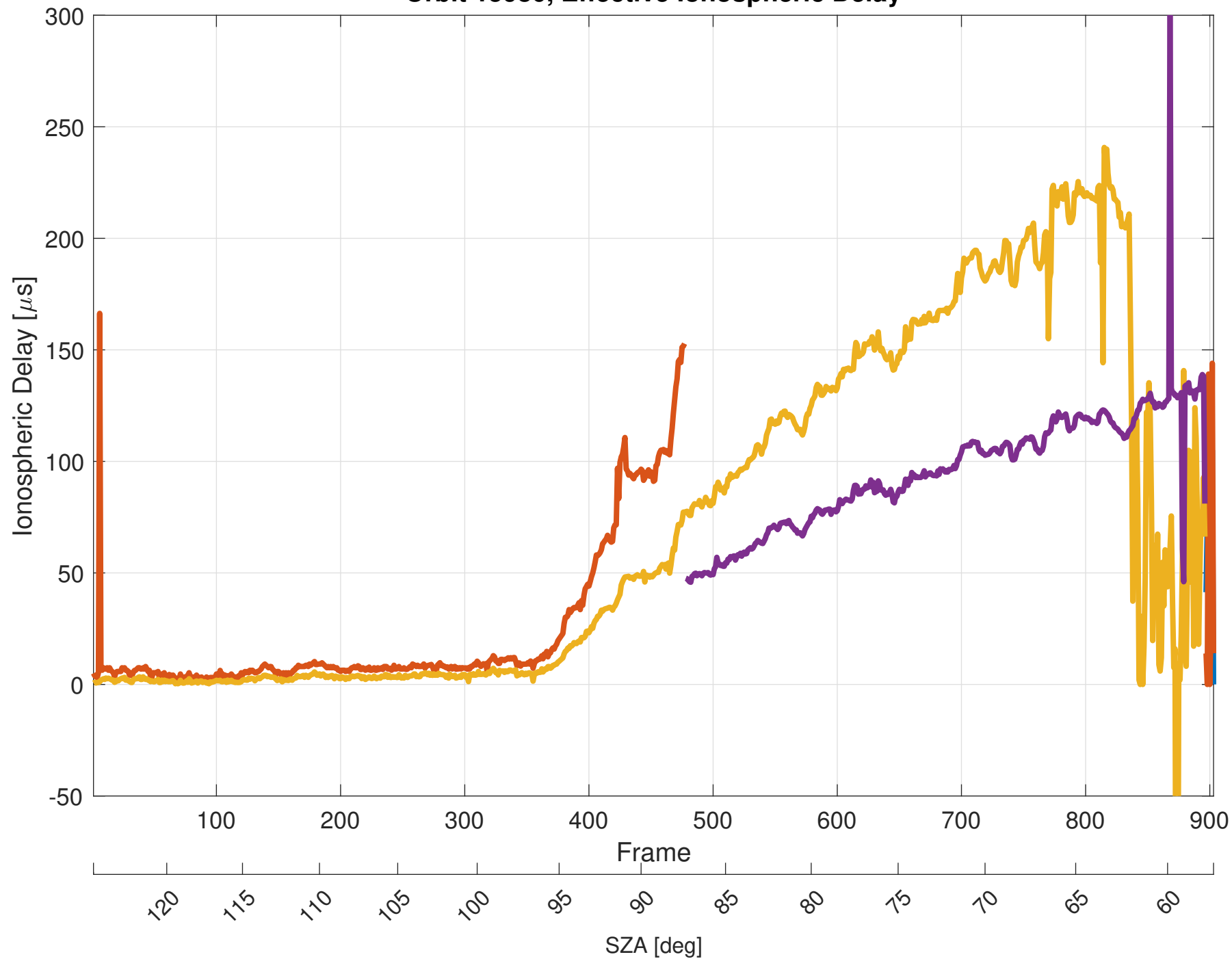
Orbit 15980, Effective Ionospheric Delay
