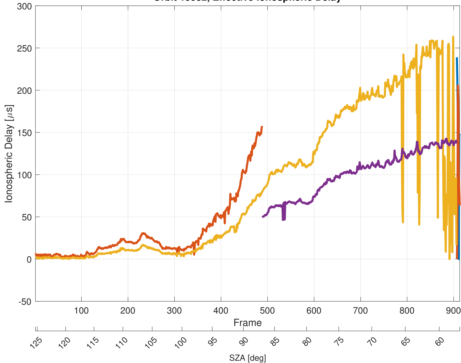
Orbit 15982, Effective Ionospheric Delay
