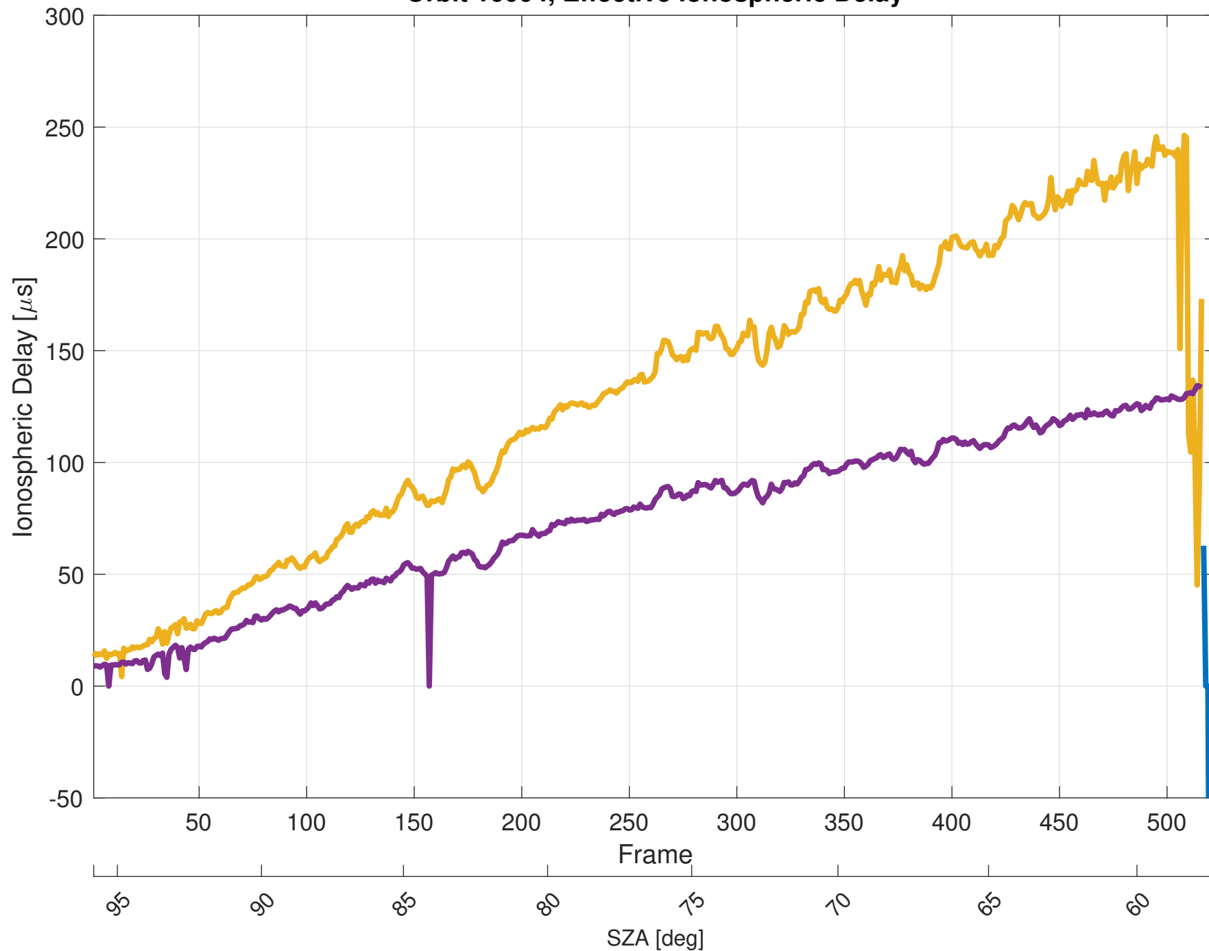
Orbit 16004, Effective Ionospheric Delay
