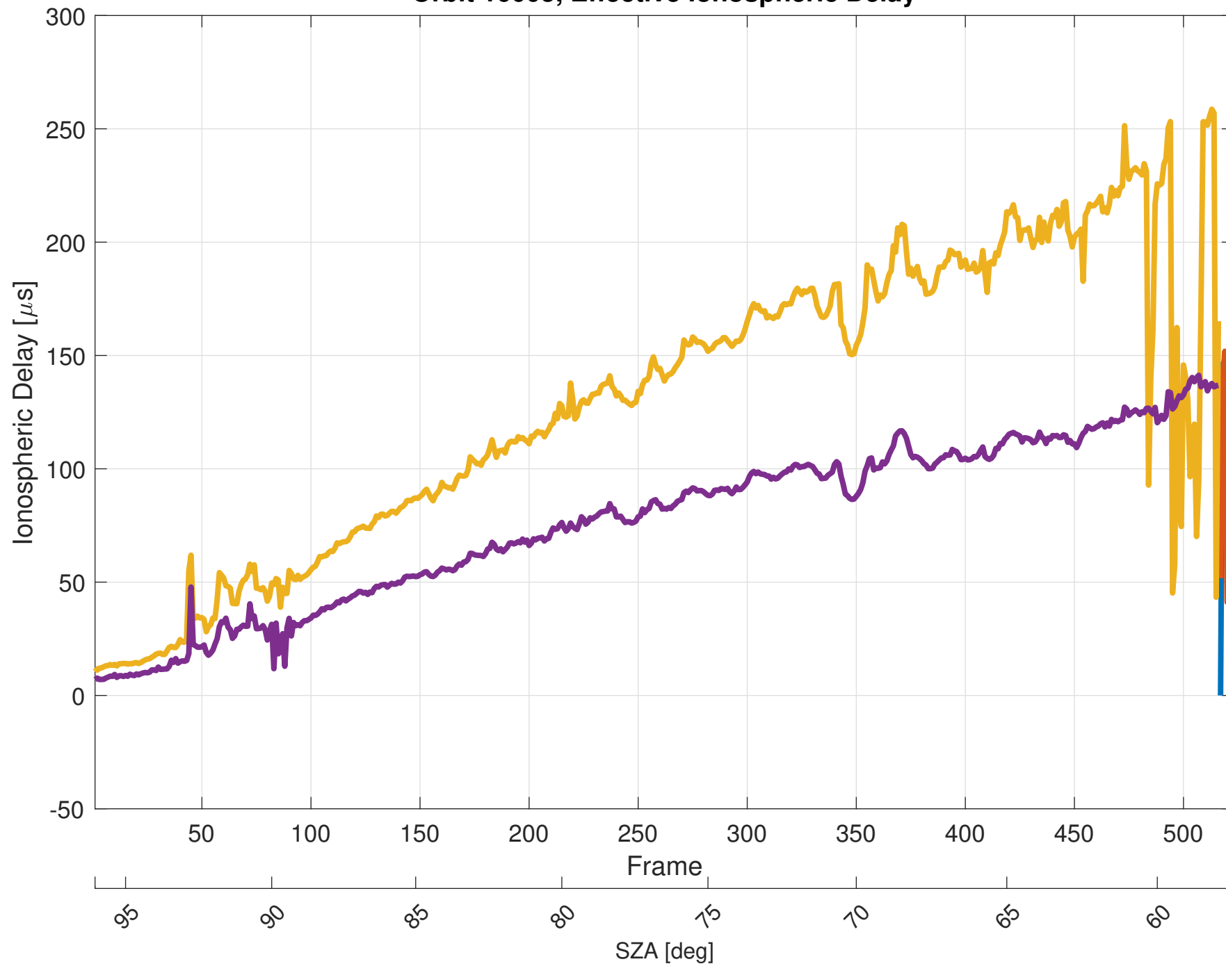
Orbit 16005, Effective Ionospheric Delay
