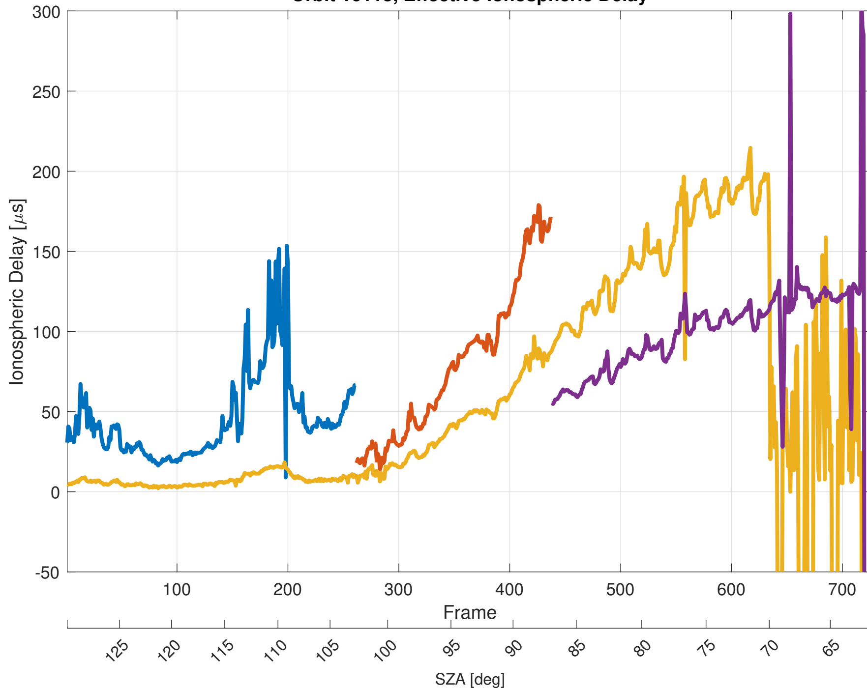
Orbit 16113, Effective Ionospheric Delay
