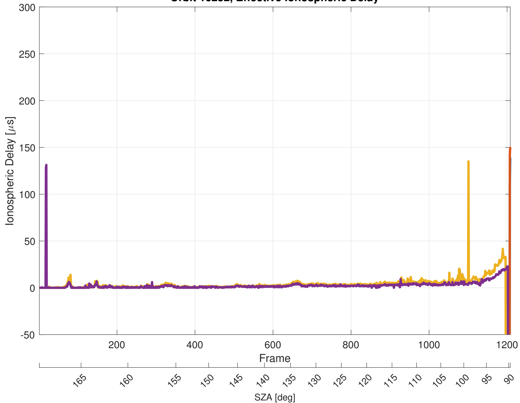
Orbit 16232, Effective Ionospheric Delay
