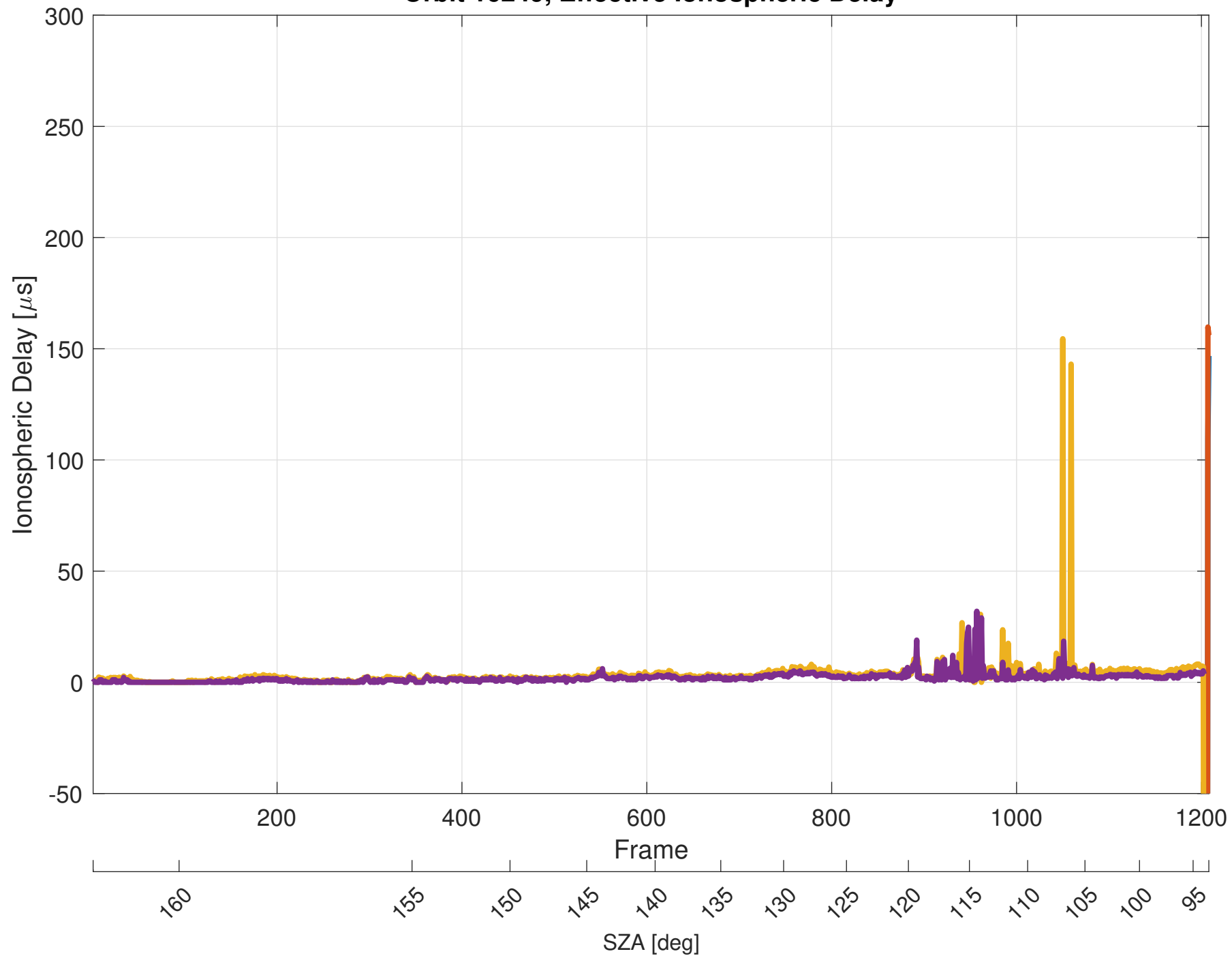
Orbit 16249, Effective Ionospheric Delay
