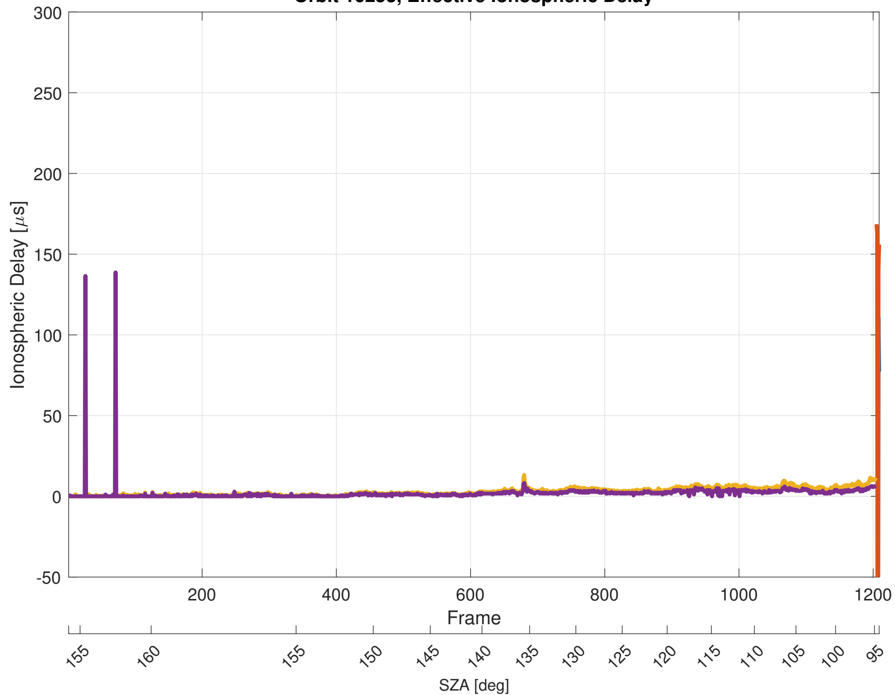
Orbit 16253, Effective Ionospheric Delay
