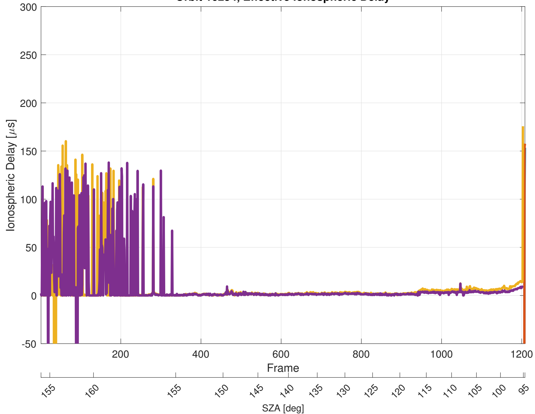
Orbit 16254, Effective Ionospheric Delay
