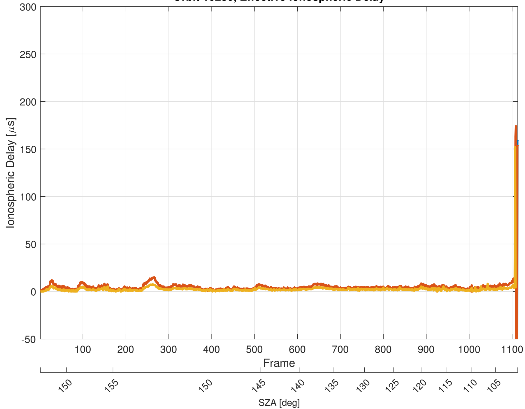
Orbit 16280, Effective Ionospheric Delay
