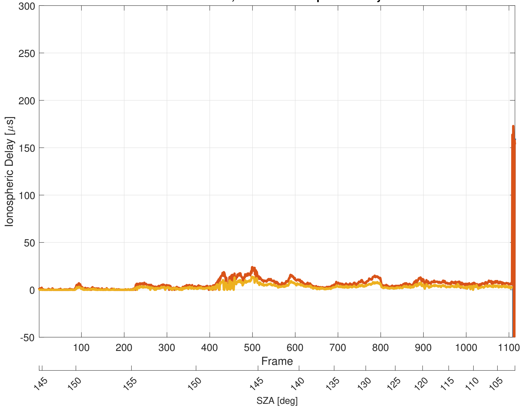
Orbit 16285, Effective Ionospheric Delay
