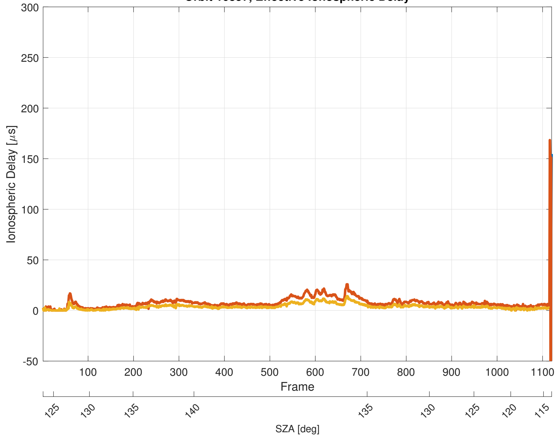
Orbit 16357, Effective Ionospheric Delay
