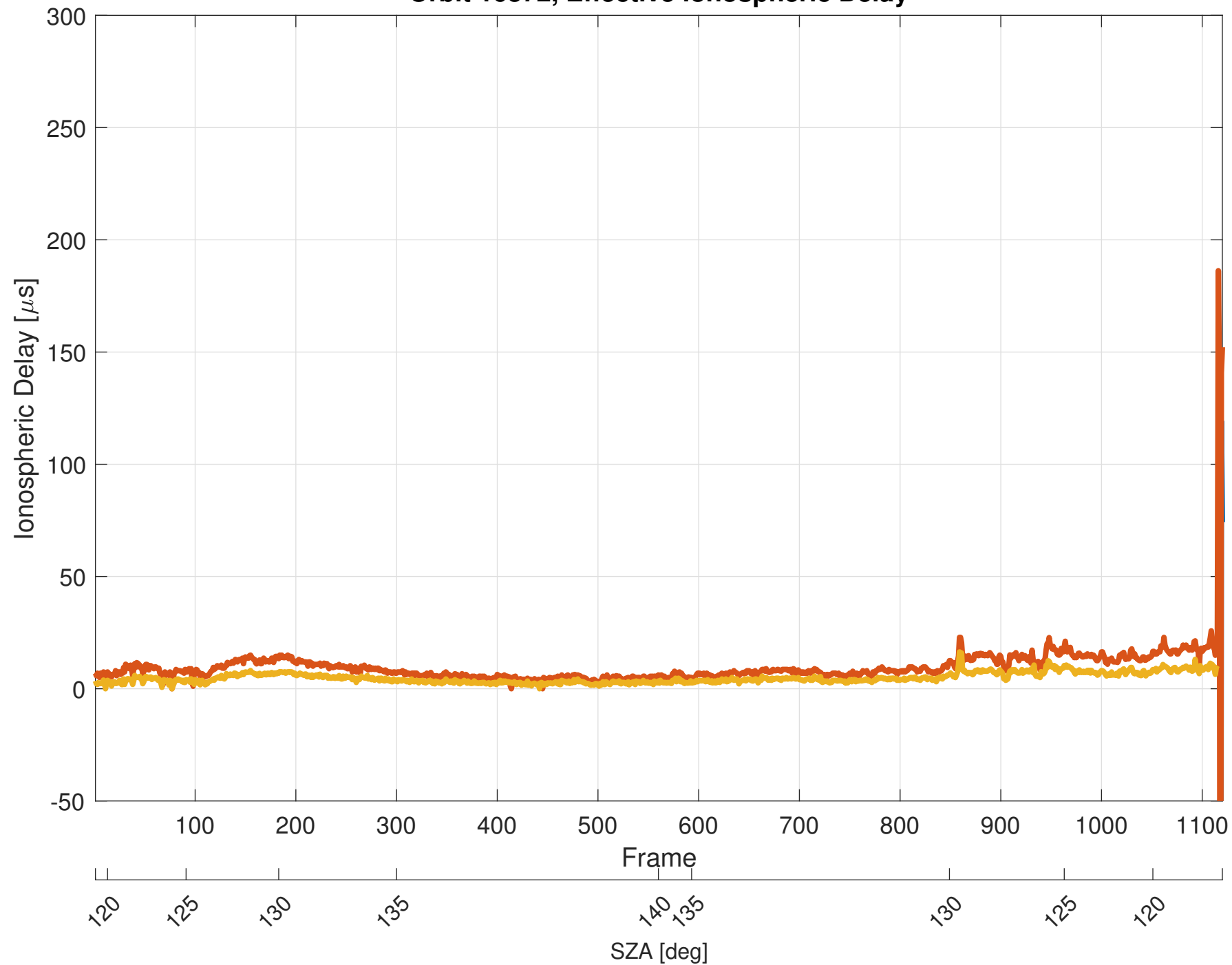
Orbit 16372, Effective Ionospheric Delay
