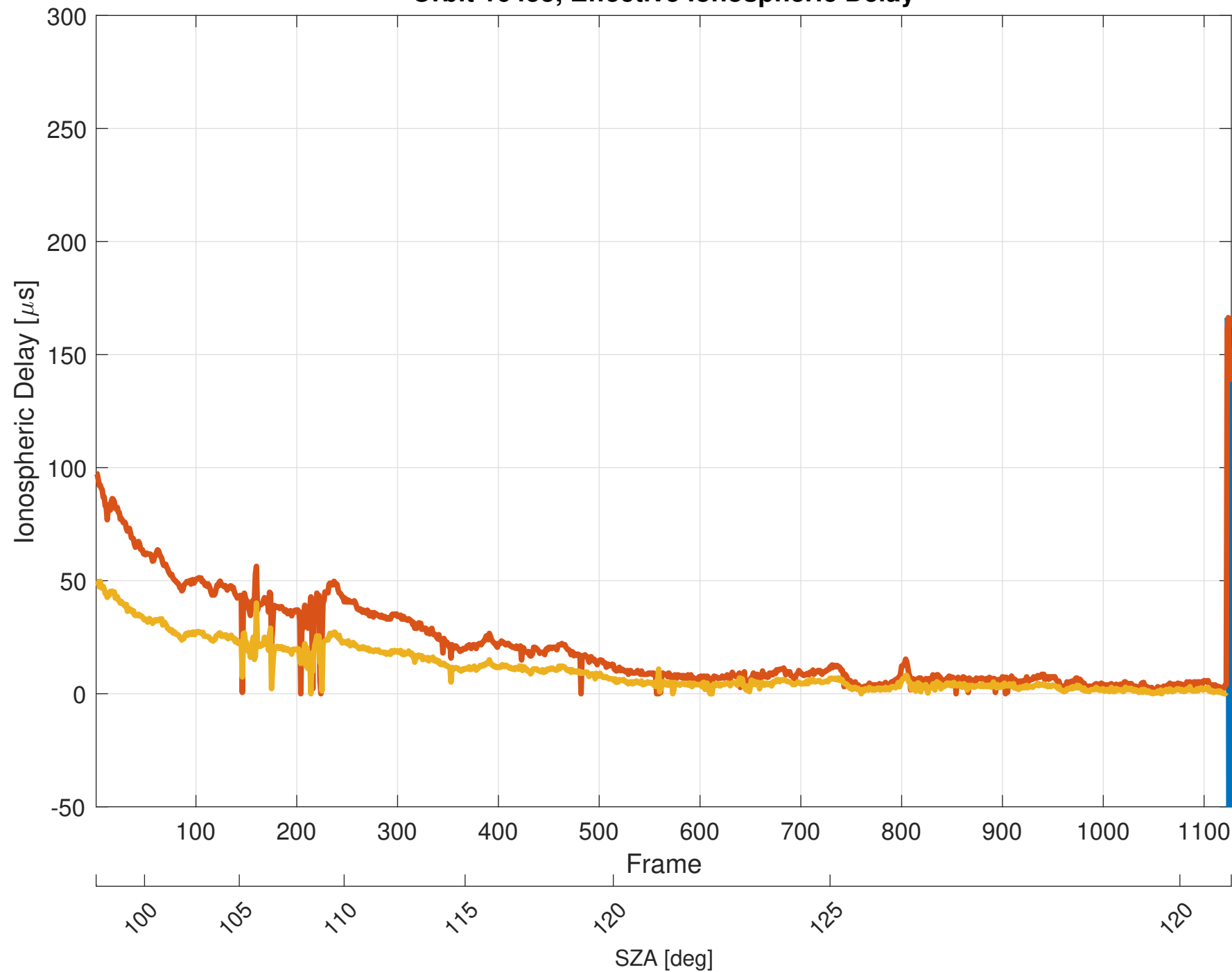
Orbit 16455, Effective Ionospheric Delay
