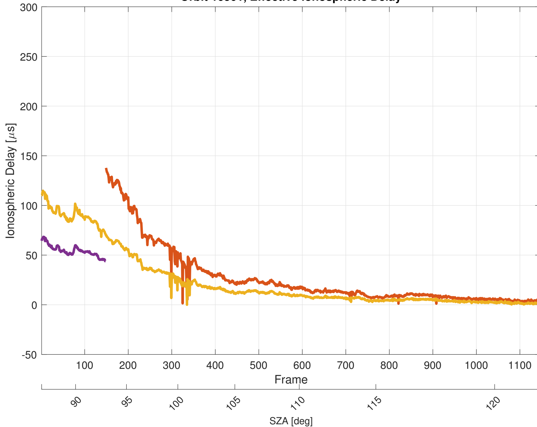
Orbit 16501, Effective Ionospheric Delay
