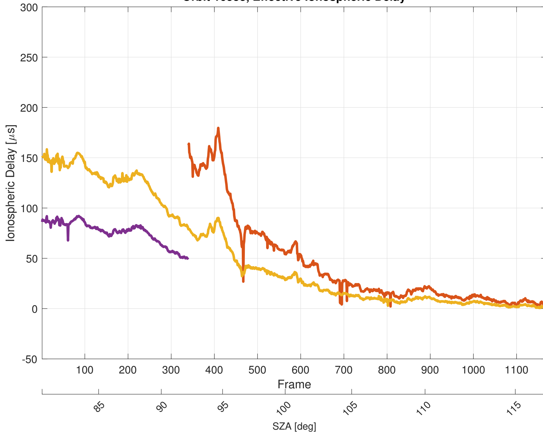
Orbit 16533, Effective Ionospheric Delay
