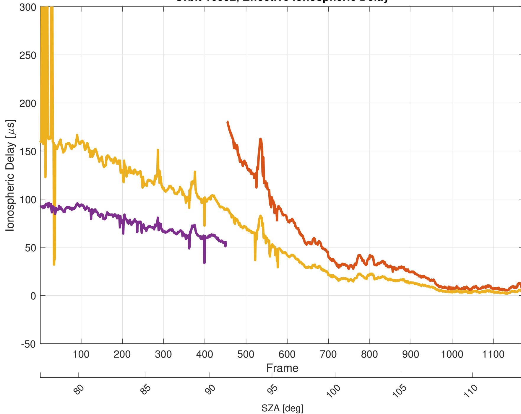
Orbit 16552, Effective Ionospheric Delay
