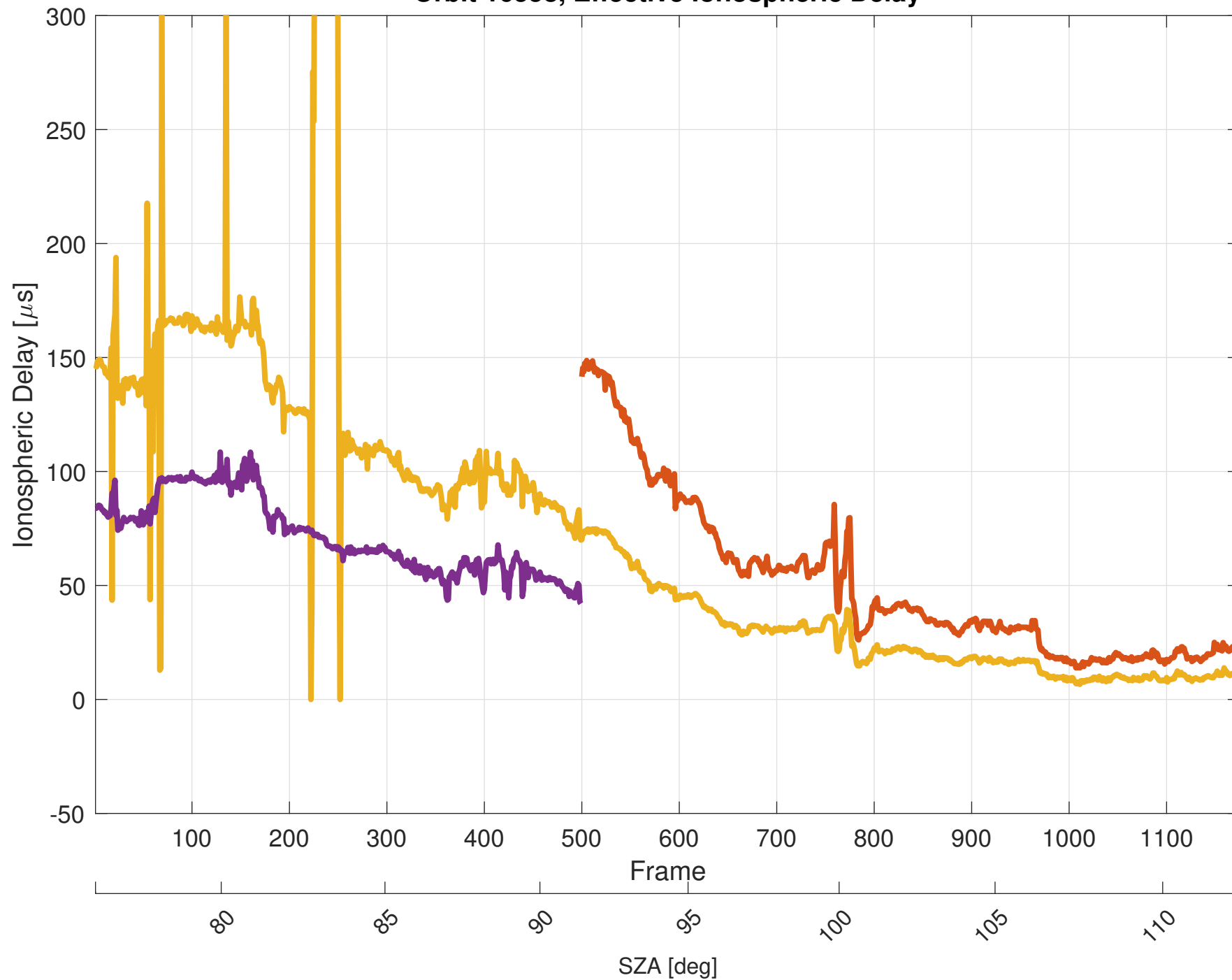
Orbit 16558, Effective Ionospheric Delay
