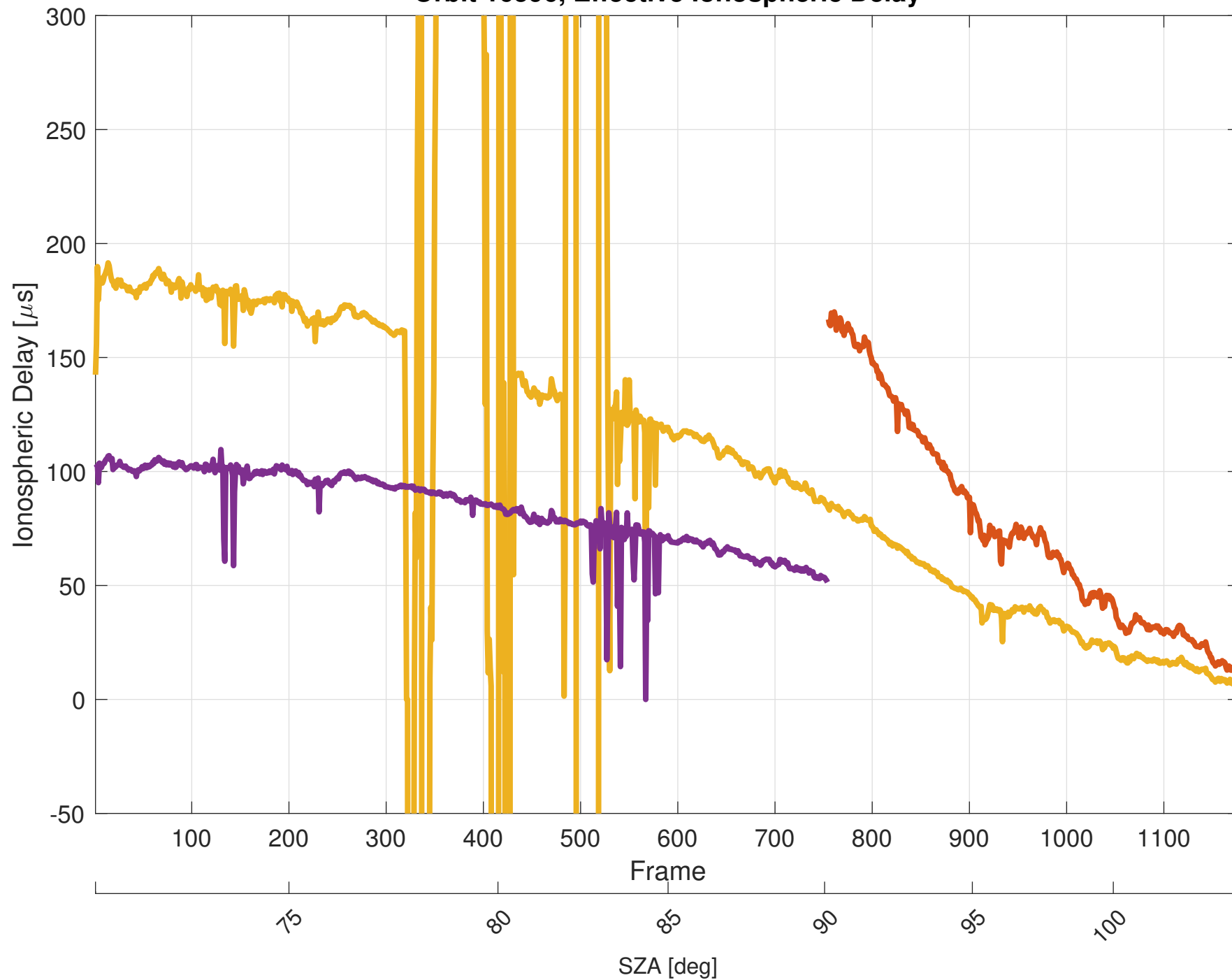
Orbit 16596, Effective Ionospheric Delay
