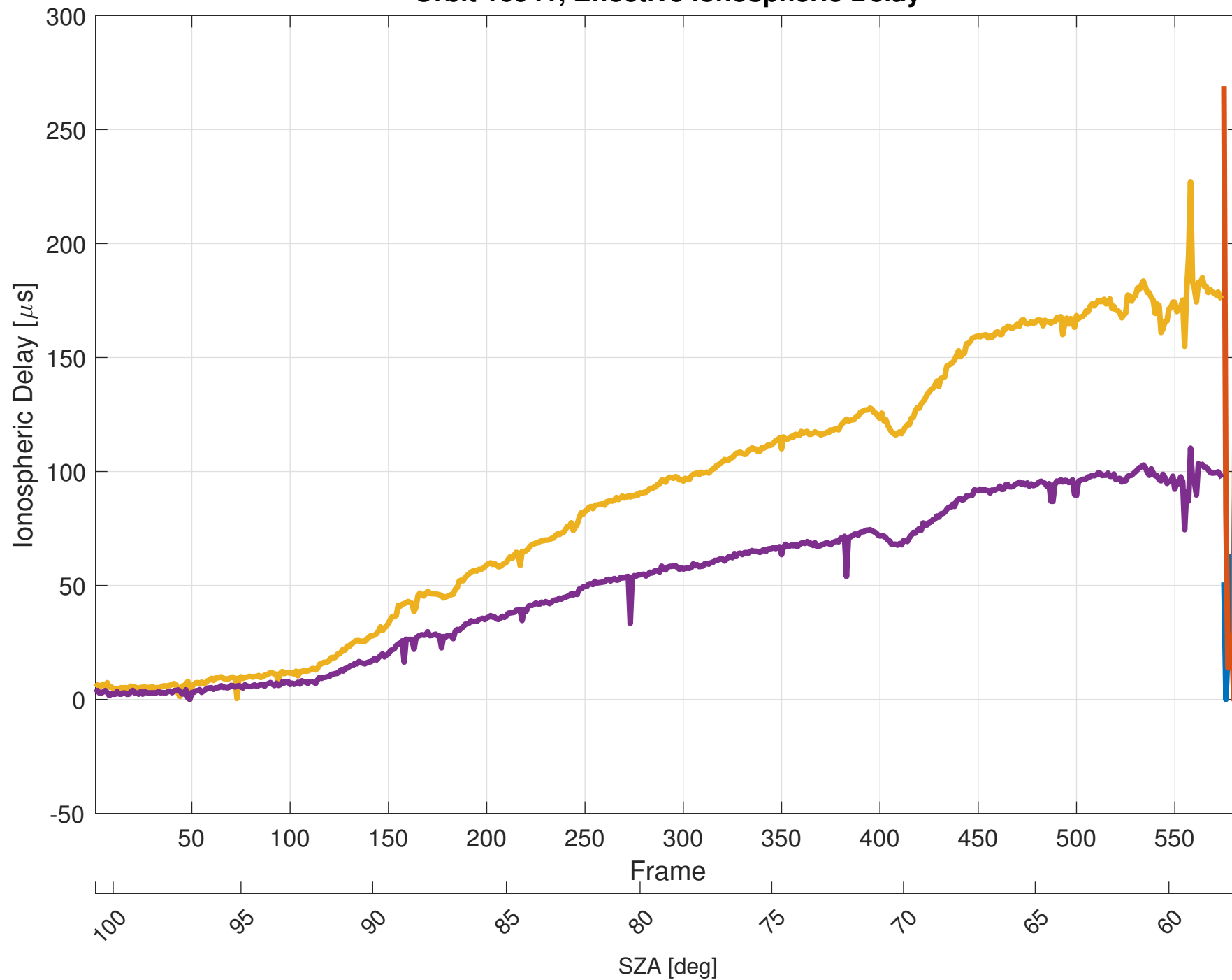
Orbit 16941, Effective Ionospheric Delay
