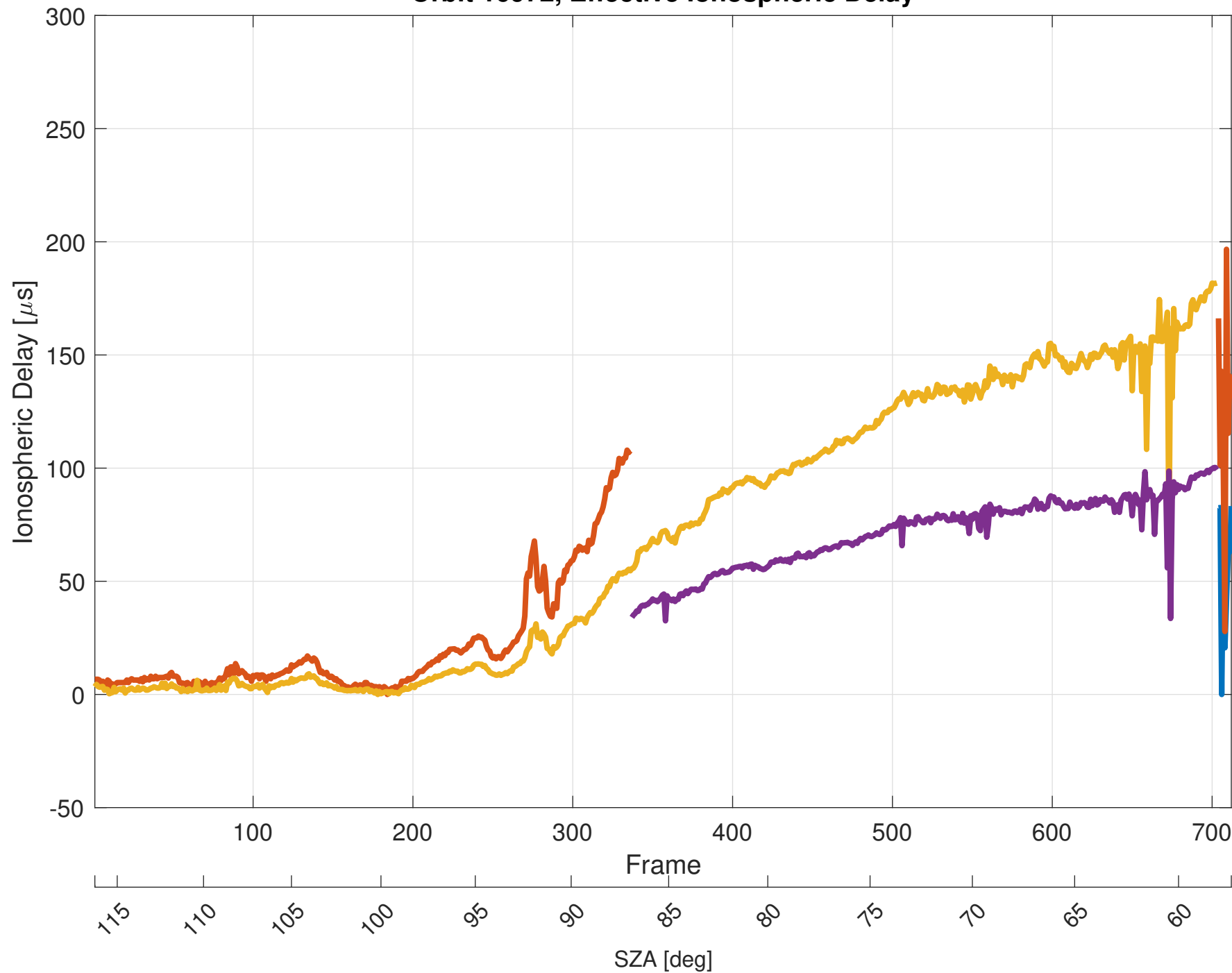
Orbit 16972, Effective Ionospheric Delay
