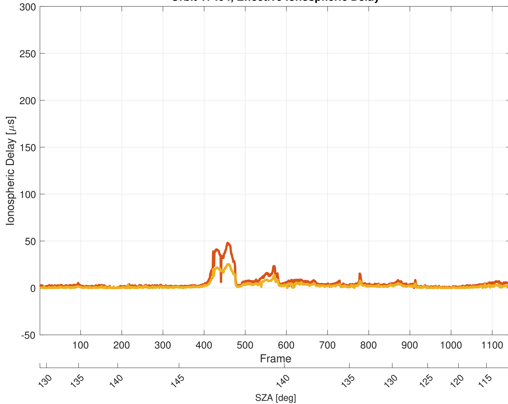
Orbit 17404, Effective Ionospheric Delay
