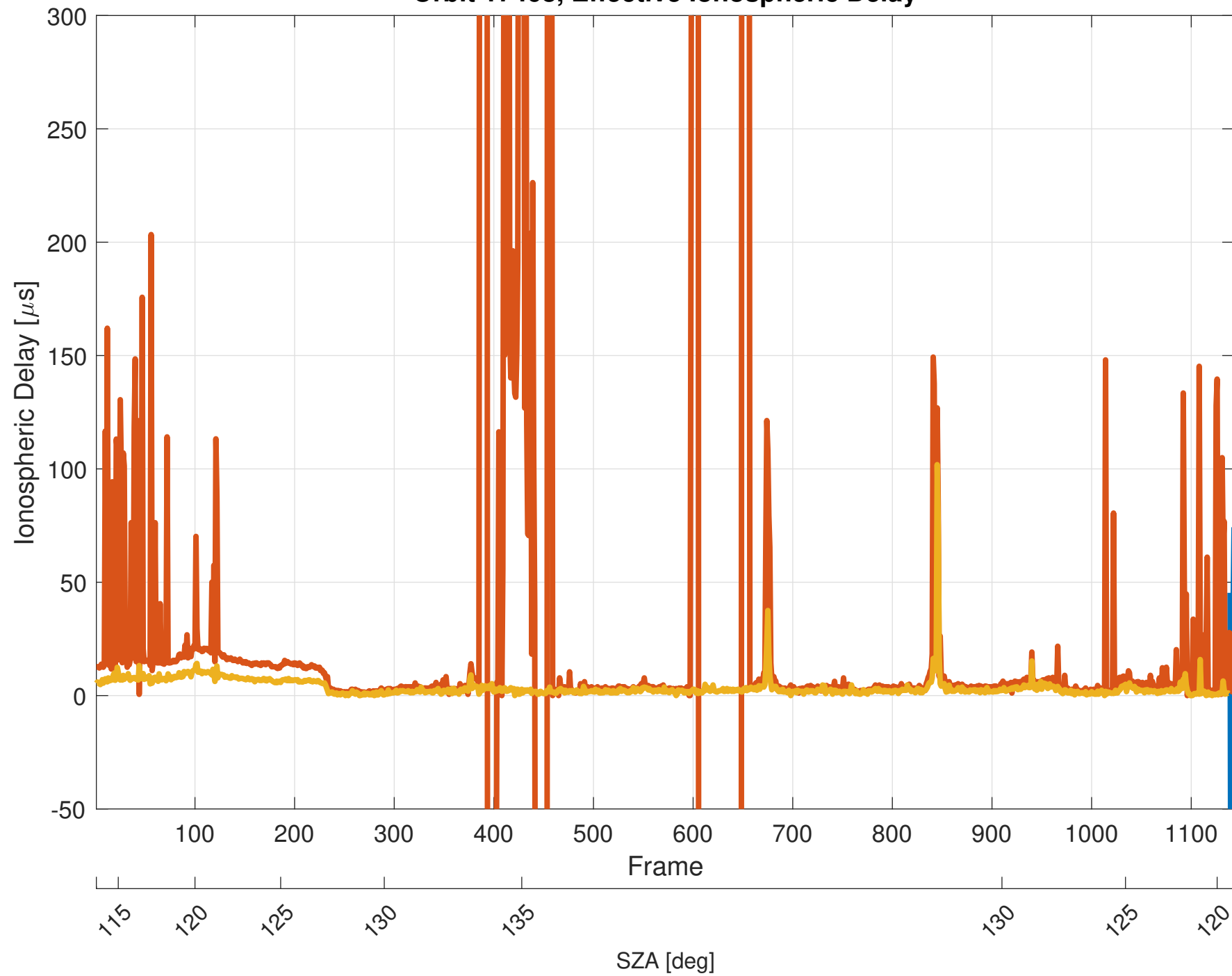
Orbit 17468, Effective Ionospheric Delay
