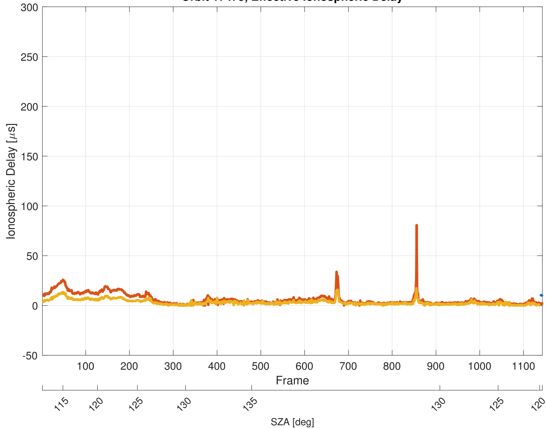
Orbit 17475, Effective Ionospheric Delay
