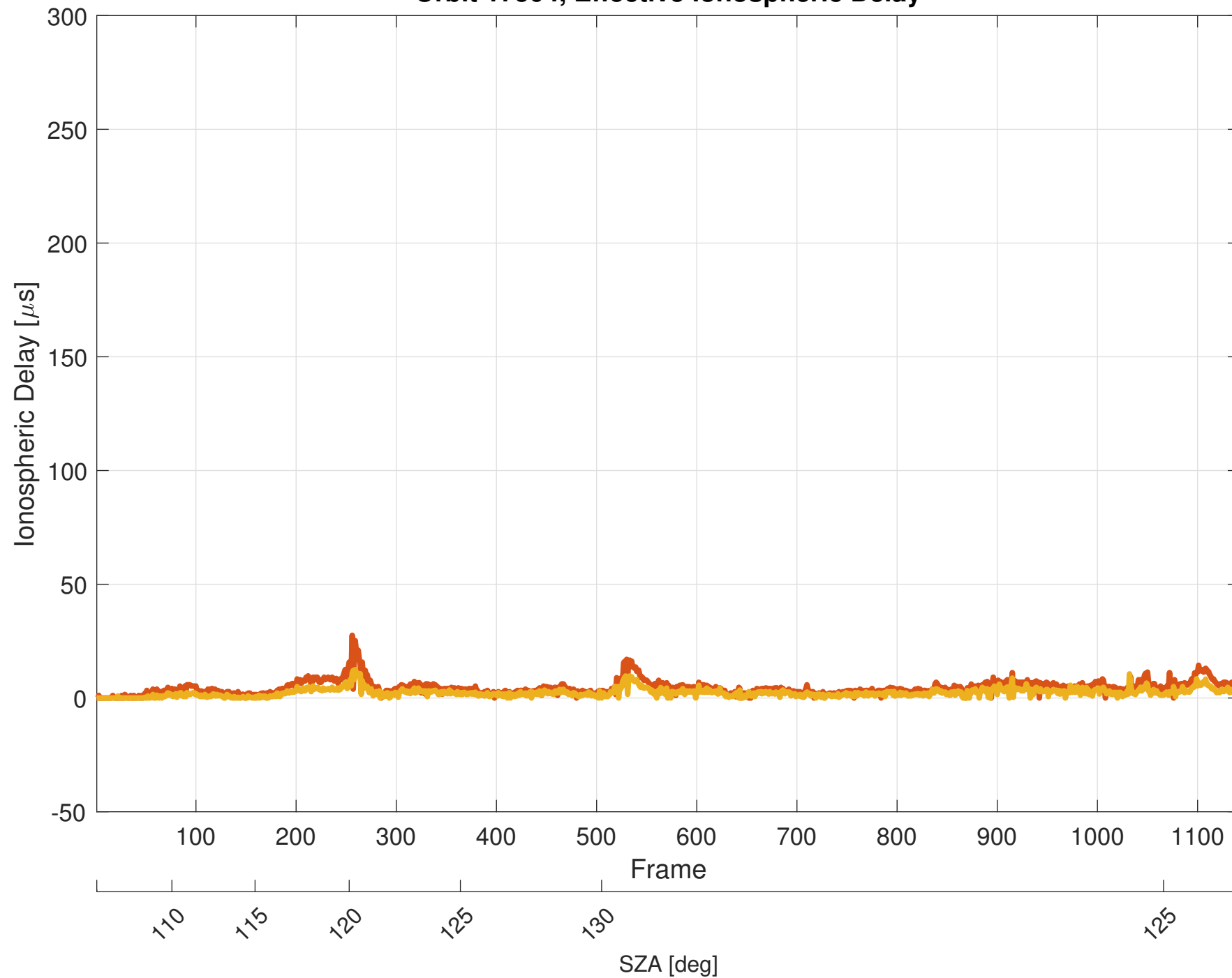
Orbit 17504, Effective Ionospheric Delay
