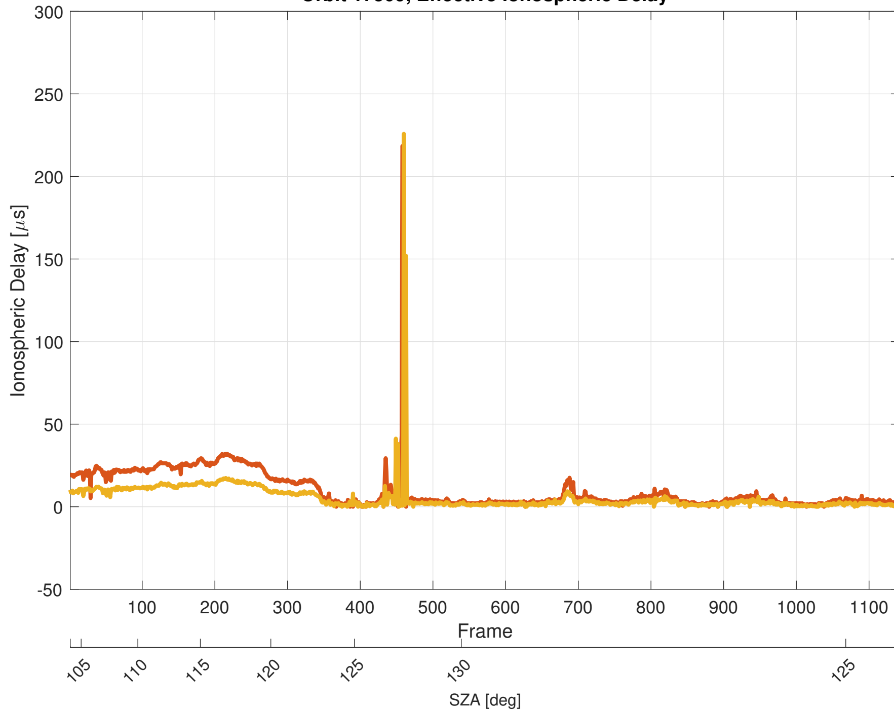
Orbit 17509, Effective Ionospheric Delay
