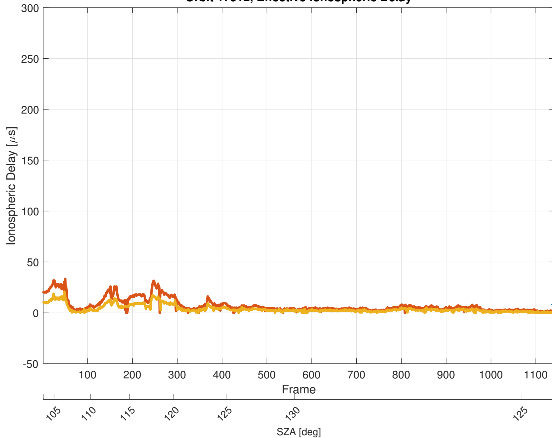
Orbit 17512, Effective Ionospheric Delay
