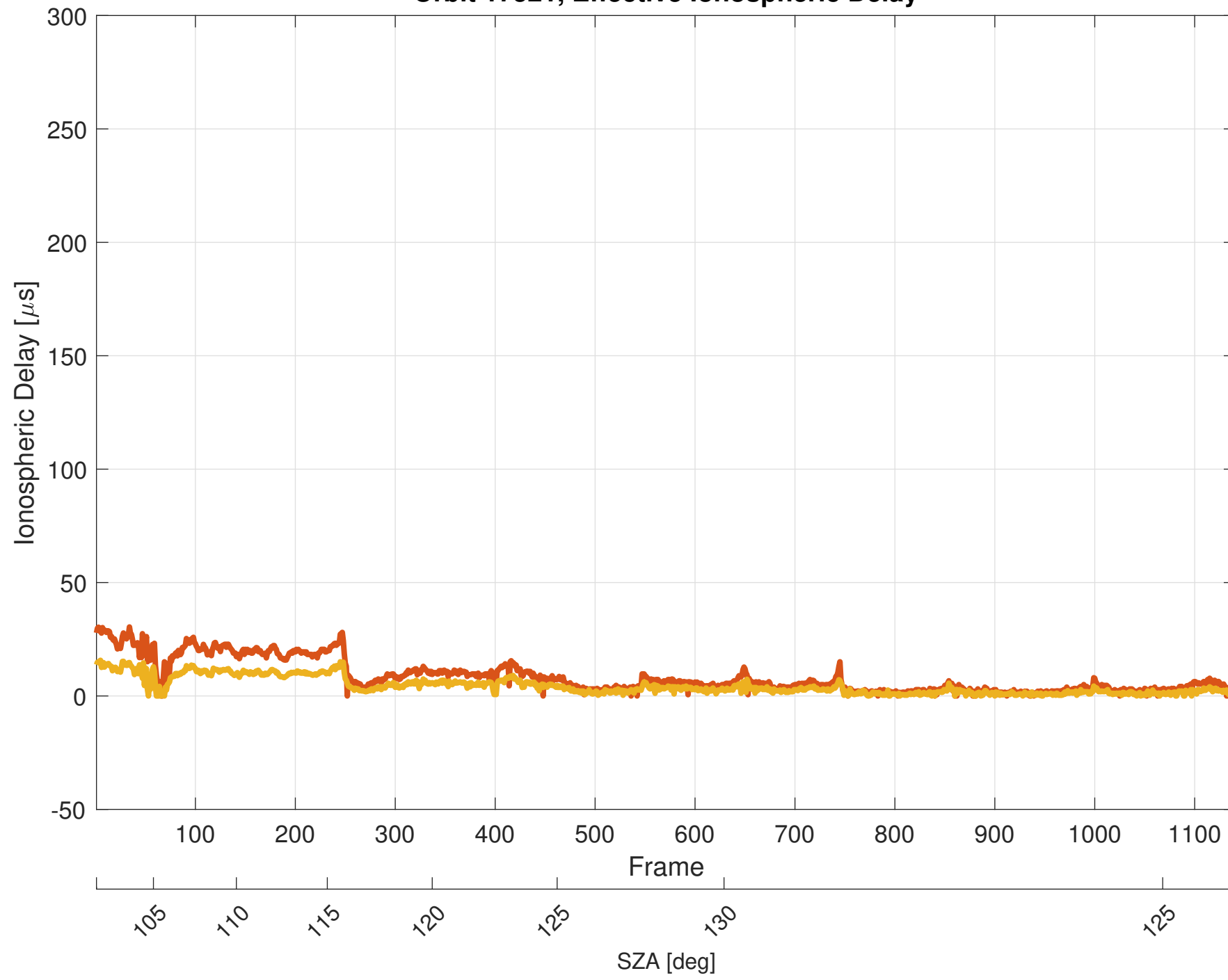
Orbit 17521, Effective Ionospheric Delay
