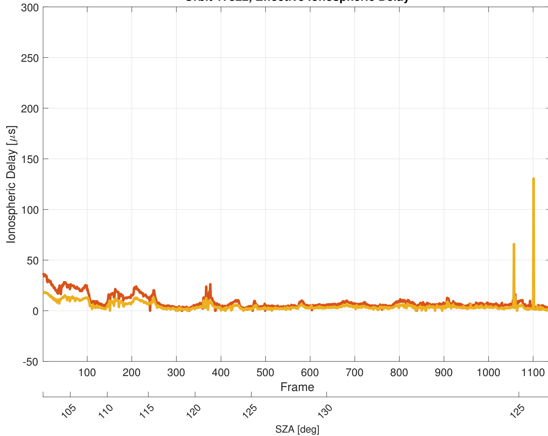
Orbit 17522, Effective Ionospheric Delay
