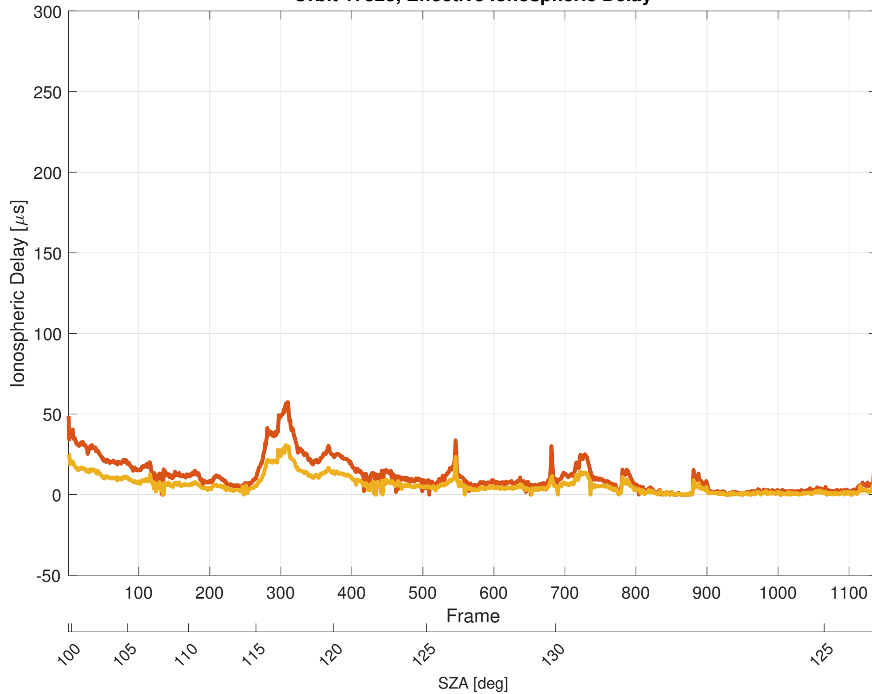
Orbit 17528, Effective Ionospheric Delay
