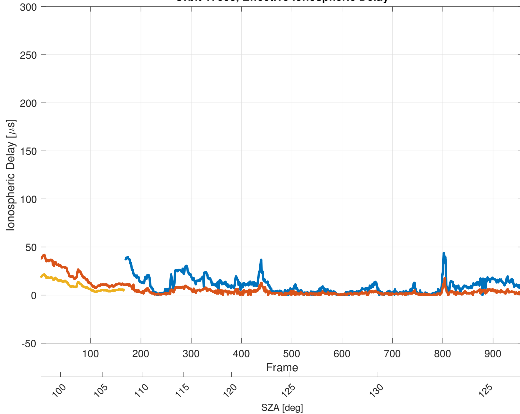
Orbit 17538, Effective Ionospheric Delay
