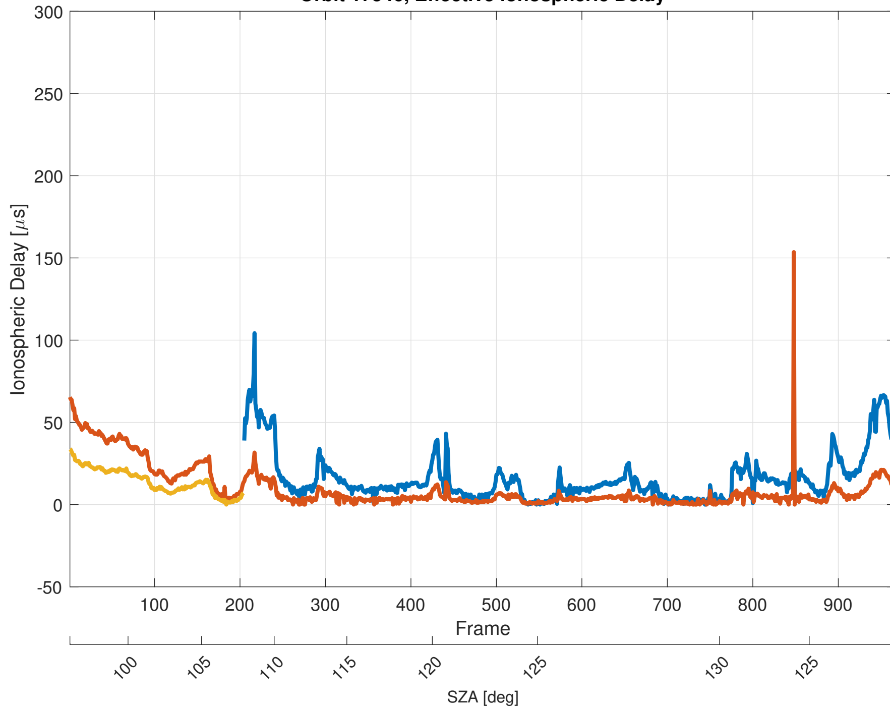
Orbit 17546, Effective Ionospheric Delay
