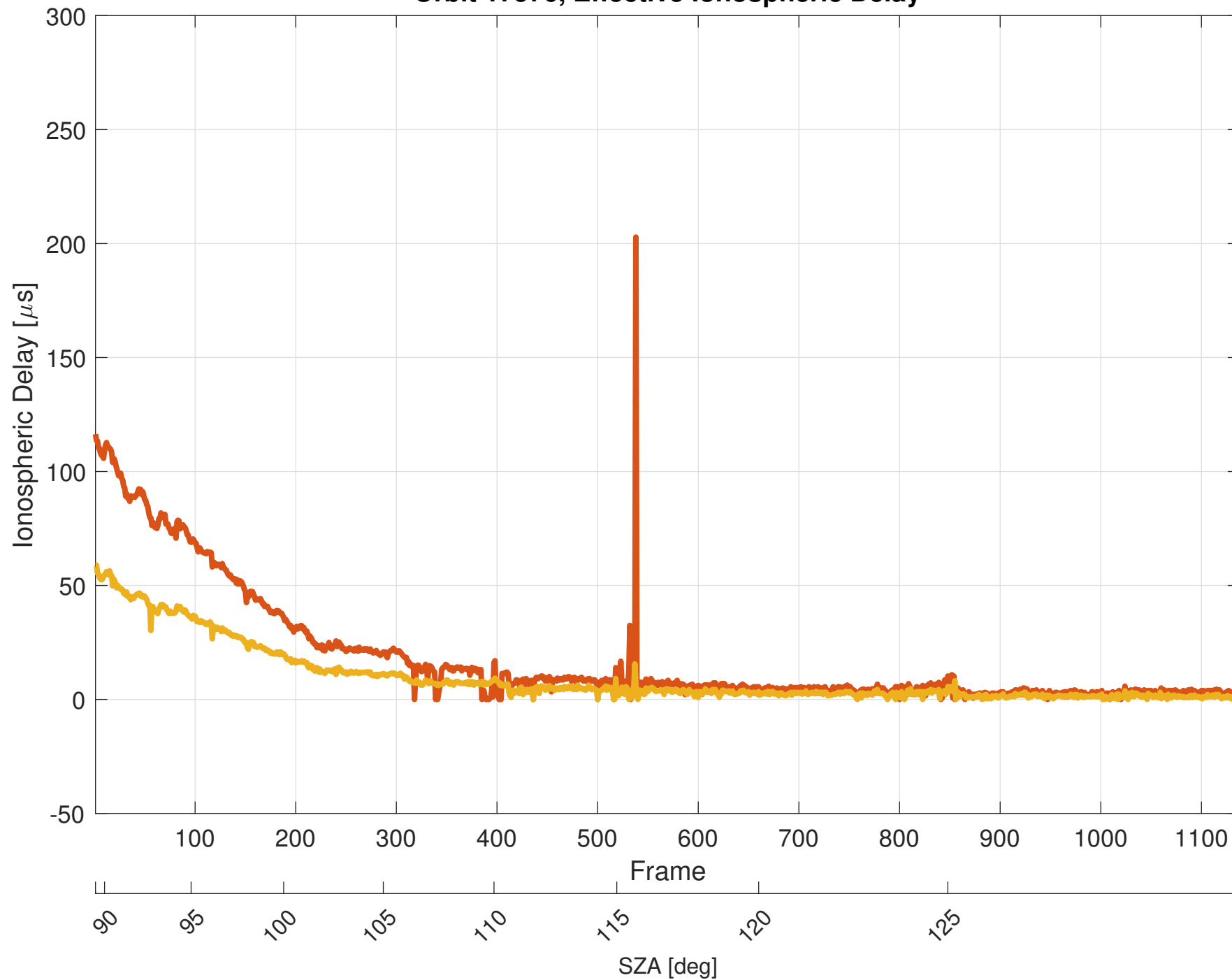
Orbit 17576, Effective Ionospheric Delay
