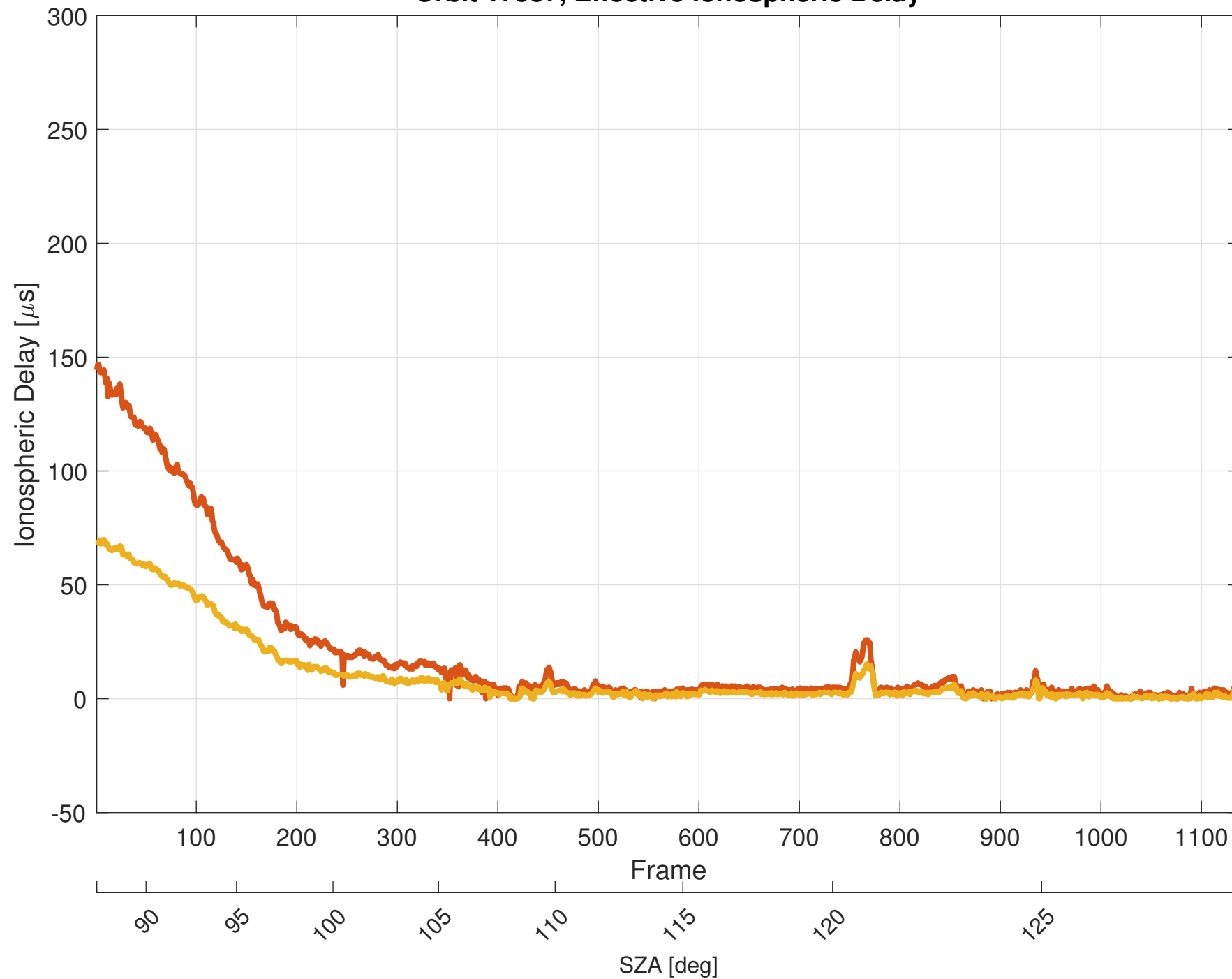
Orbit 17587, Effective Ionospheric Delay
