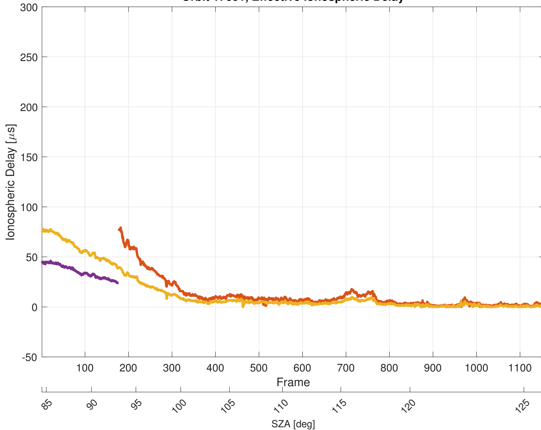
Orbit 17601, Effective Ionospheric Delay
