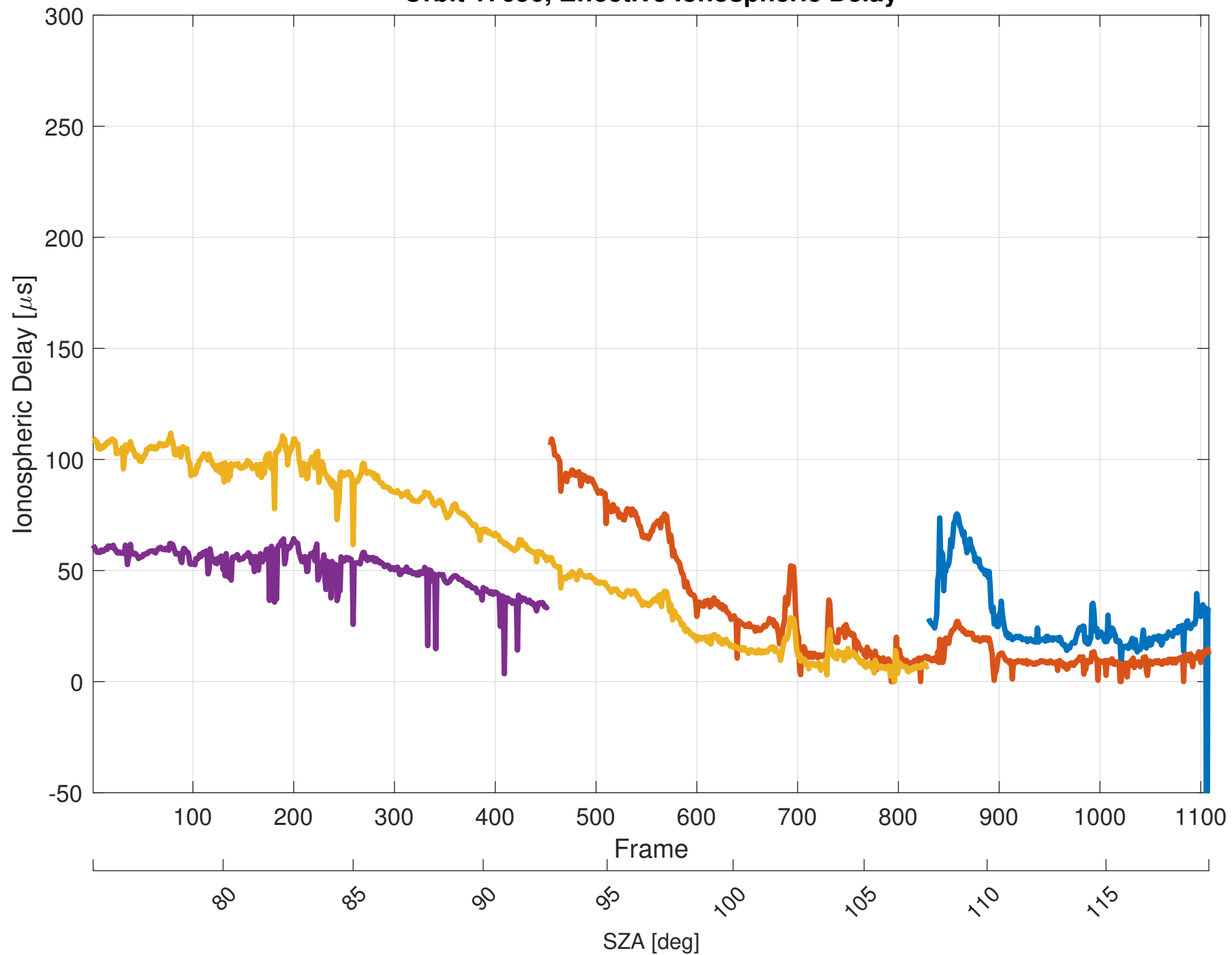
Orbit 17656, Effective Ionospheric Delay
